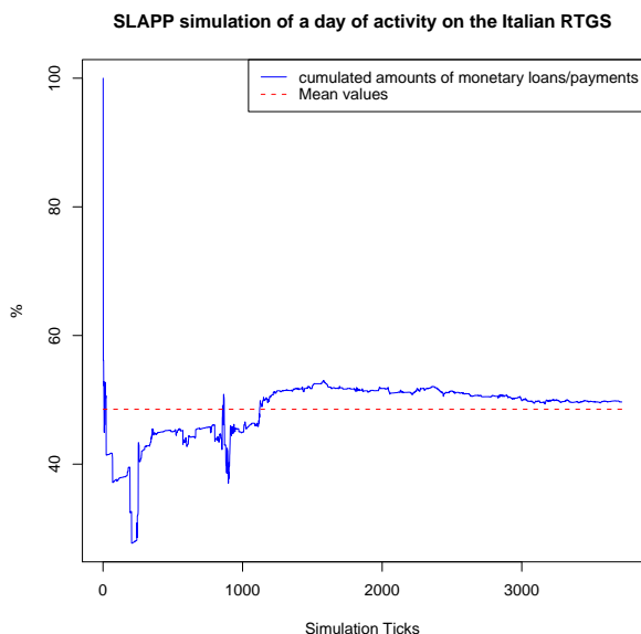
Figure 2: SLAPP simulation of a day of activity on the Italian RTGS system. Ratio between cumulated amounts of monetary market loans and payments.
