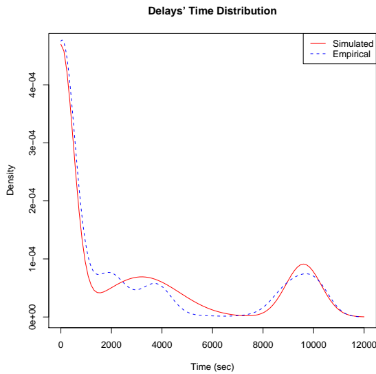
Figure 5: In the graph are plotted the empirical (blue dashed line) and the simulated (red line) time distribution of the delays.
