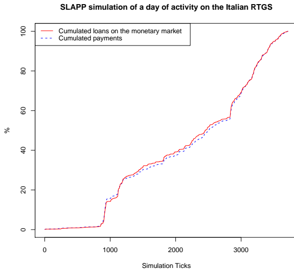
Figure 1: SLAPP simulation of a day of activity on the Italian RTGS system. Cumulated percentage amounts of payments (blue dashed line) and monetary market loans (red line).
